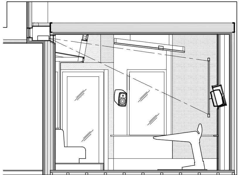
CONTROL ROOM SECTION
